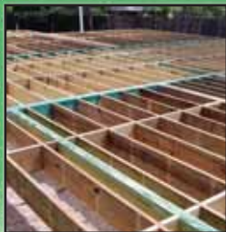
Raised Floor
